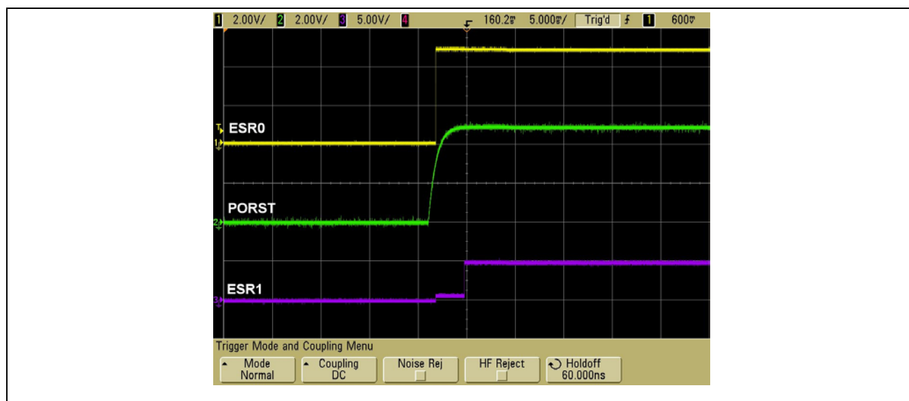
Figure 8 ESR1 as Reset Out Signal with Reset Out Delay after Power-up
