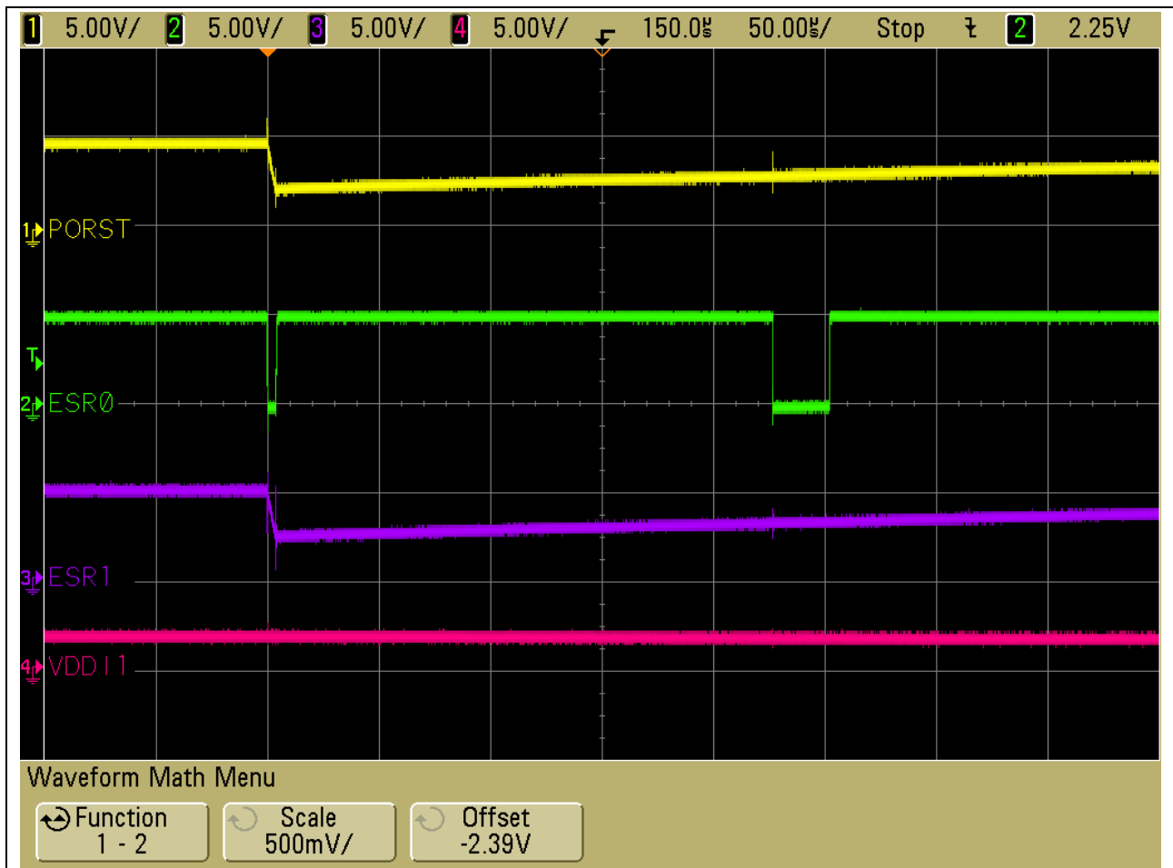
Figure 6 Trigger a PORST with the ESR1 Pin
