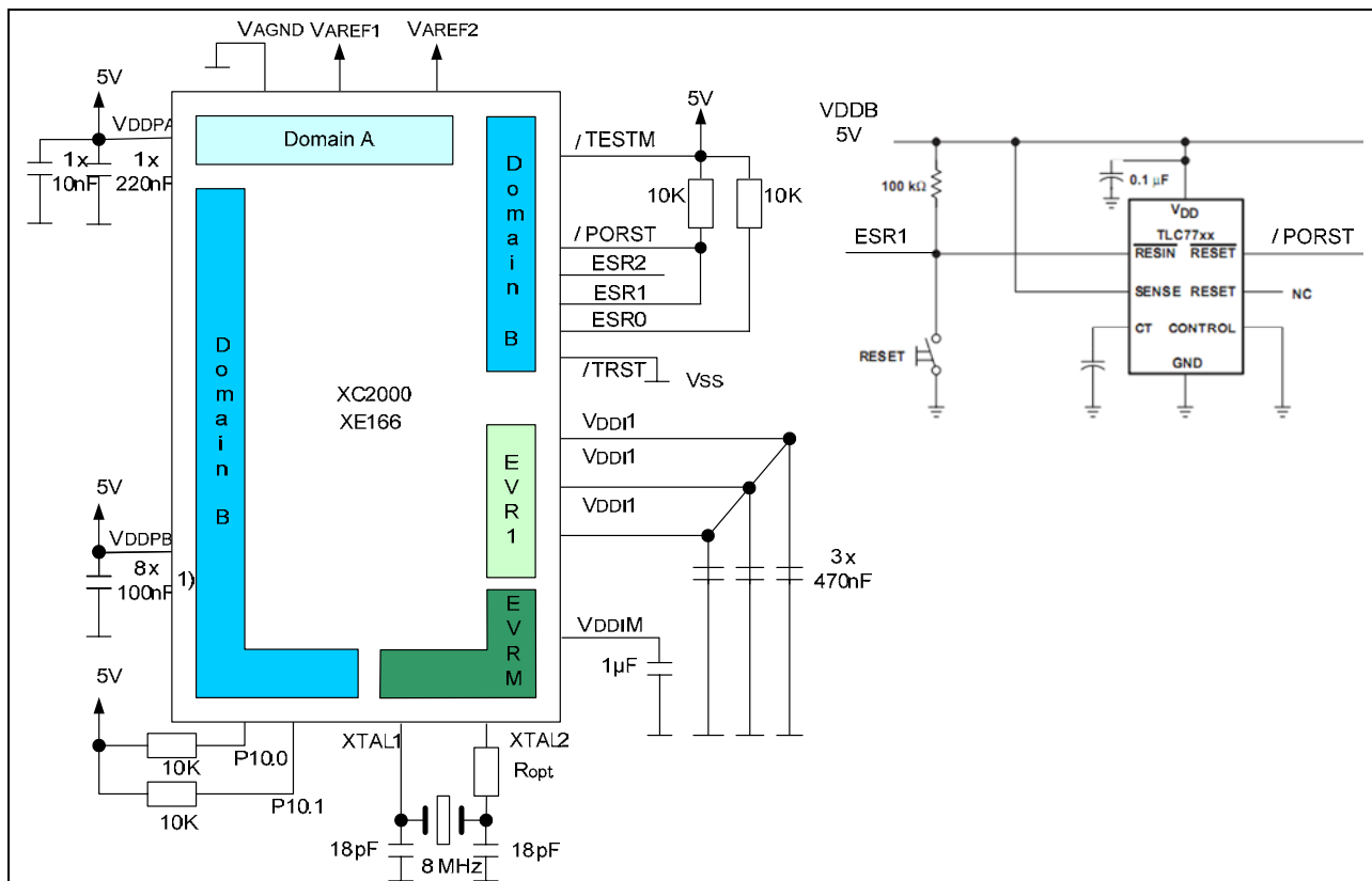
Figure 5 Trigger a PORST with the ESR1 Pin
