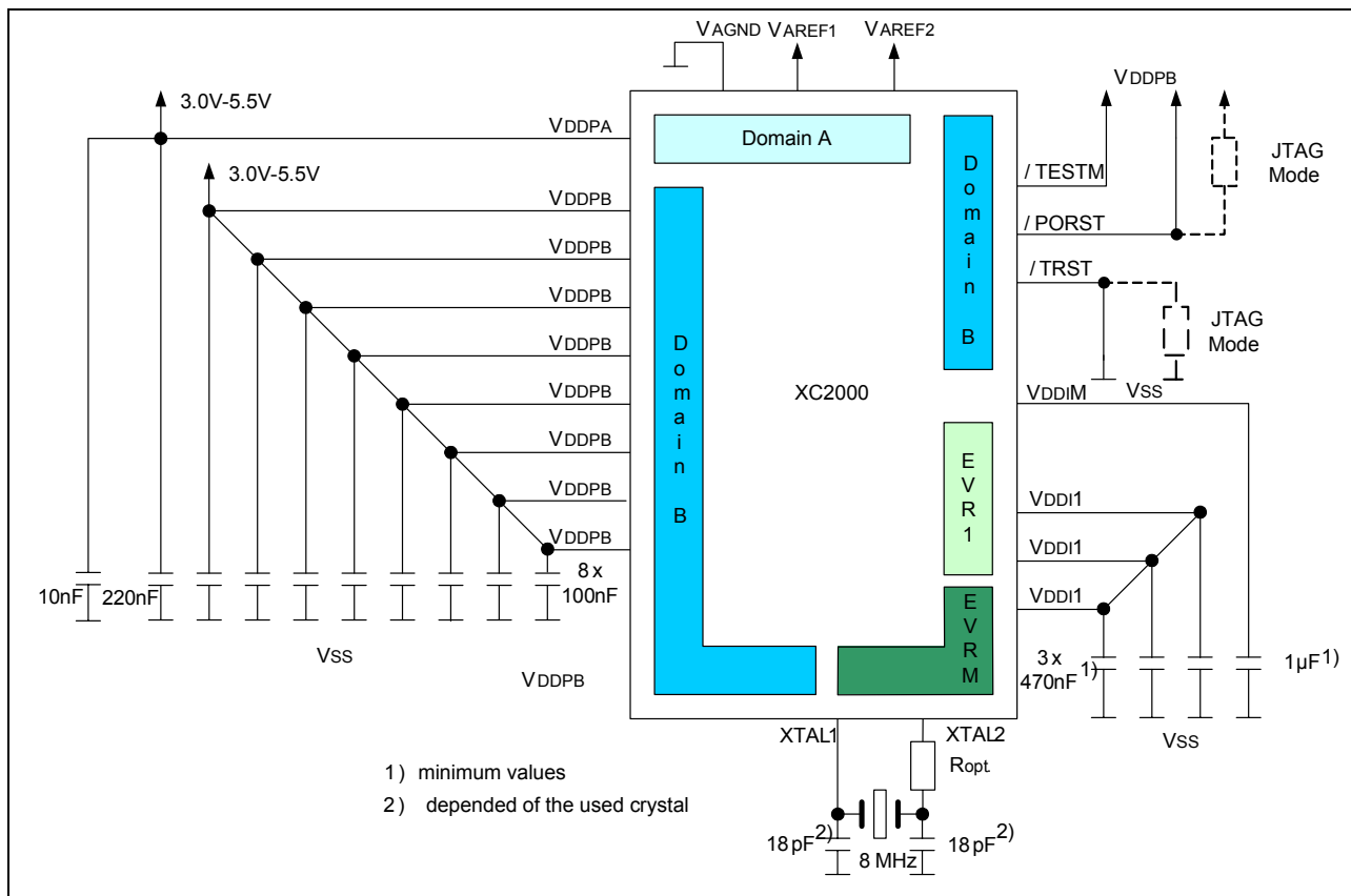
Figure 1 Start from Internal Flash
