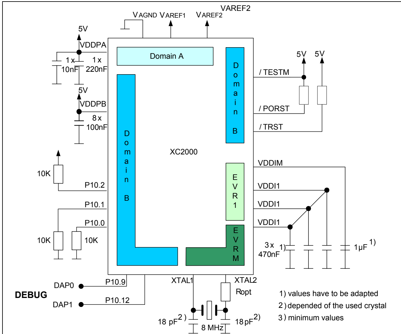
Figure 2 DAP Debug Configuration
