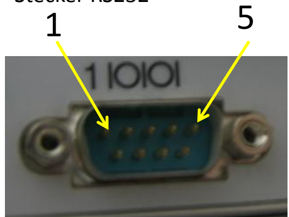
Computer RS232
