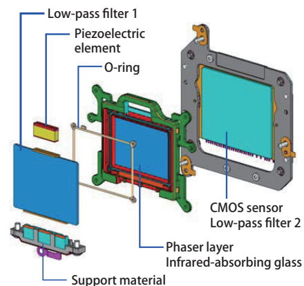
Fig. 005 Unit configuration
