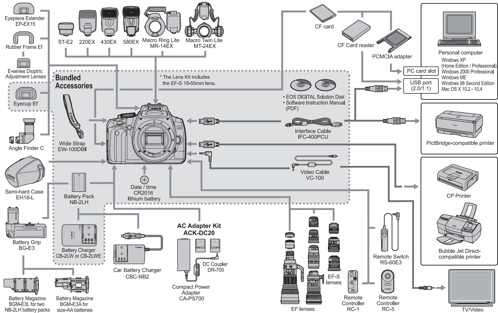
Fig. 037 System map
