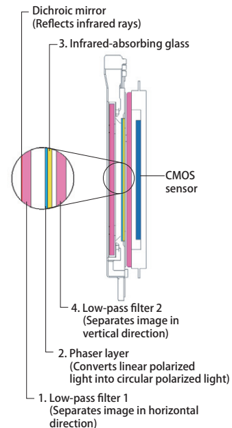
Fig. 002 Cross section of infrared cut, low-pass filter
