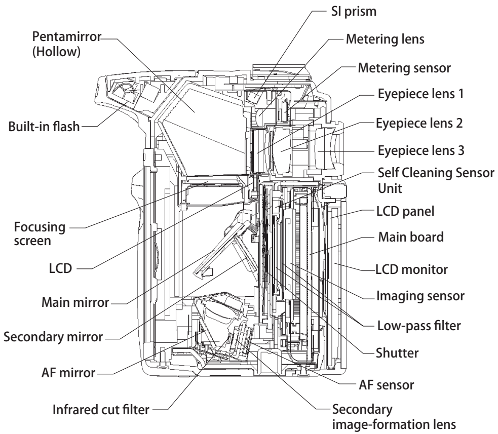
Fig. 030 Cross section at center
