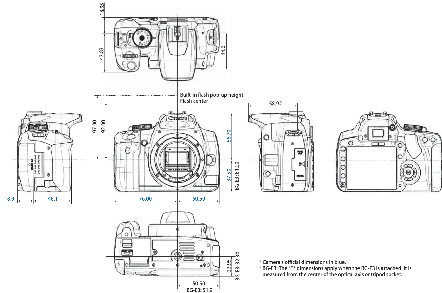
Fig. 025 Six Exterior Views
