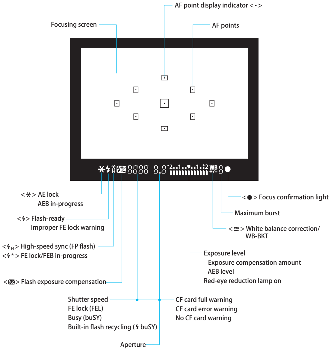
Fig. 026 Viewfinder Information
