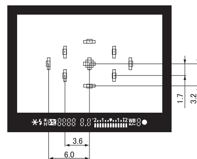
Fig. 013 Focusing area
