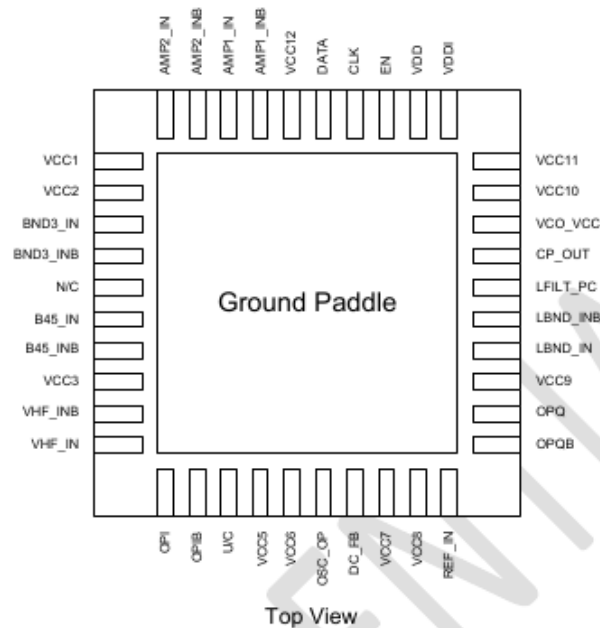
Figure 3: Pin-Out Diagram
