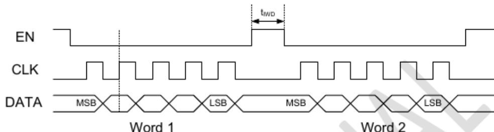
Figure 4: Serial Bus Timing Diagram
