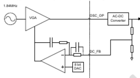
Figure 7: Voltage Generator Operational Diagram
