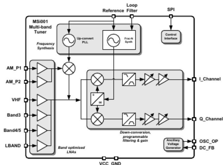
Figure 1: MSi001 Top Level Block Diagram
