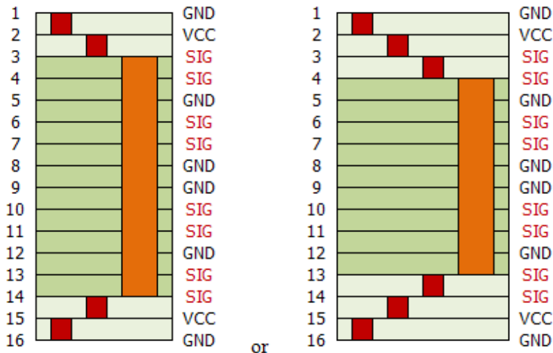
Figure 3-11: GND and VCC on outer layers
