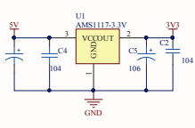
3.3V regulator
