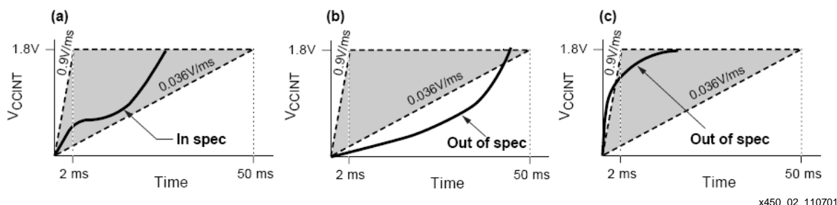
Figure 2: Spartan-IIE Ramp Time Specifications
