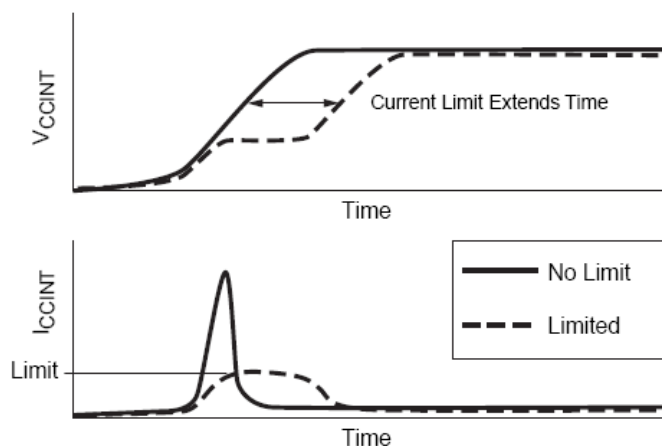
Figure 3: The Effects of a Current Limit on the POS Current
