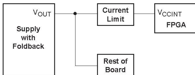
Figure 6: Limit on Power Path Avoids Foldback
