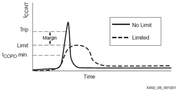
Figure 7: Selecting a Current Limit to Avoid Foldback
