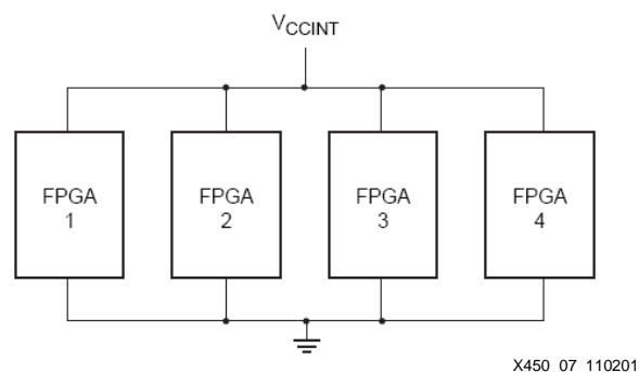
Figure 4: Multiple FPGAs During Power-On
