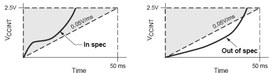
Figure 1: Spartan-II Maximum V_{CCINT} Ramp Time Specification
