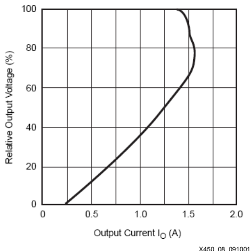
Figure 5: Regulator Foldback Characteristics
