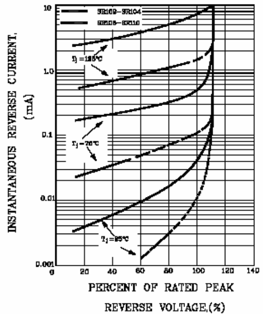
FIG.4-TYPICAL REVERSE CHARACTERISTICS
